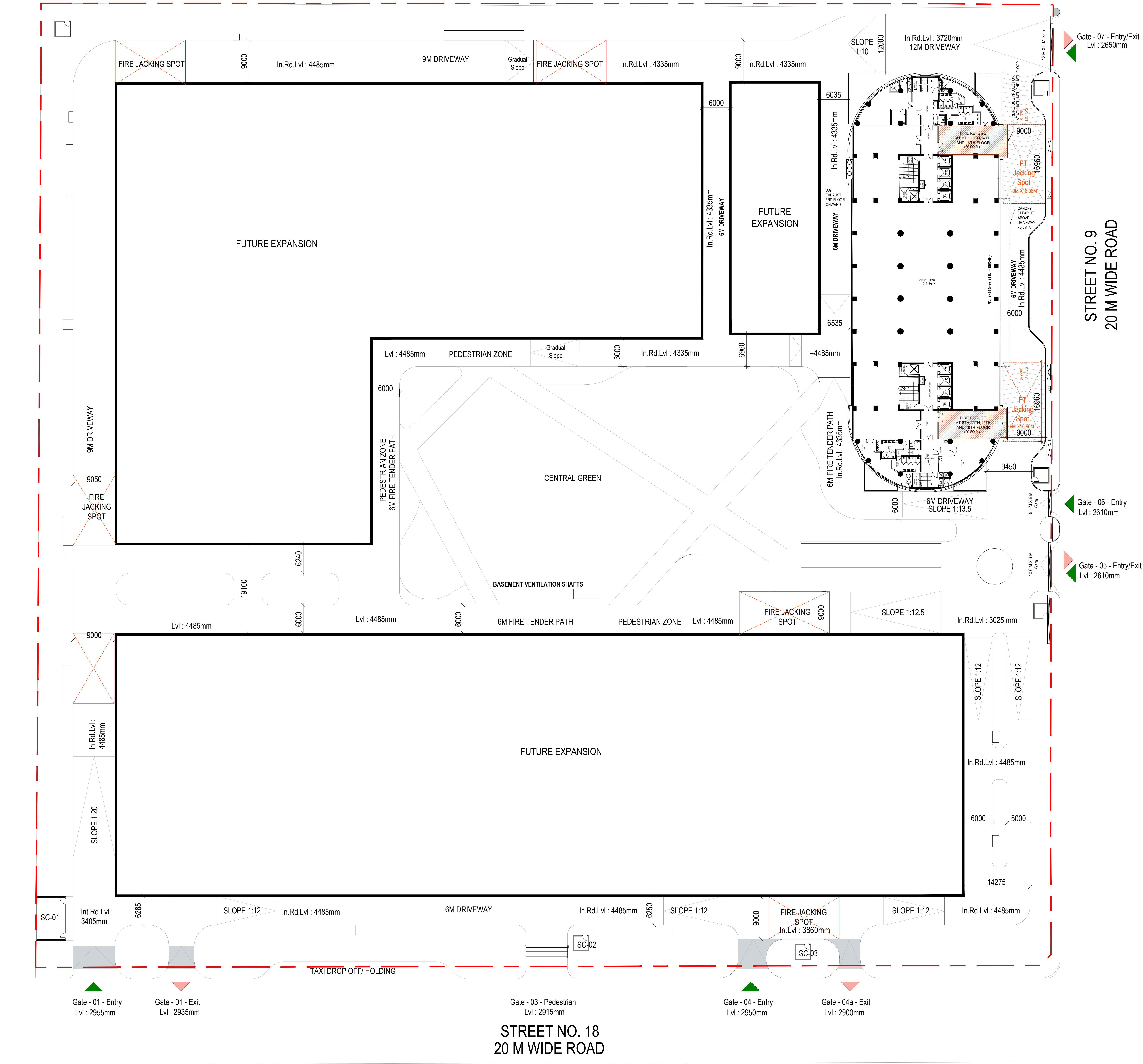
1 FIRE EVACUATION DRAWING 1 : 300
